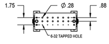
SCGB-3 - 4" x 10" w/16-Holes
