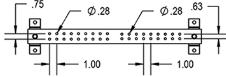
SCGB-2 - 2" x 24" w/36-Holes
