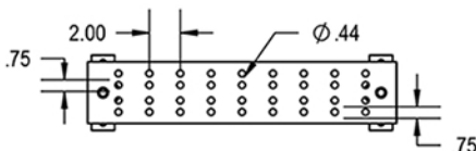
SCGB-10 - 4" x 20" 36 Holes in 4 Rows of 9
