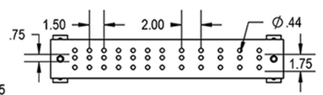
SCGB-12 - 4" x 24" 36 Holes in 4 Rows of 12
