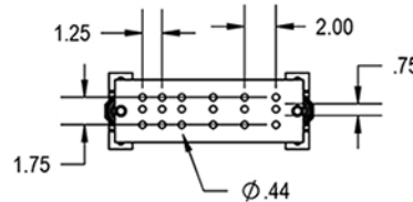
SCGB-5 - 4" x 12" w/18 Holes
