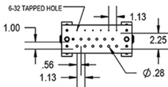
SCGB-4 - 4" x 10" 18 Holes Offset w /6 Taps
