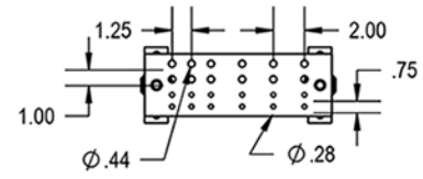
SCGB-6 - 4" x 12" 24 Holes w/6 Taps
