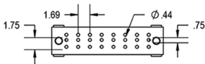
SCGB-7 - 4" x 16" 24 Holes in 3 Rows of 8
